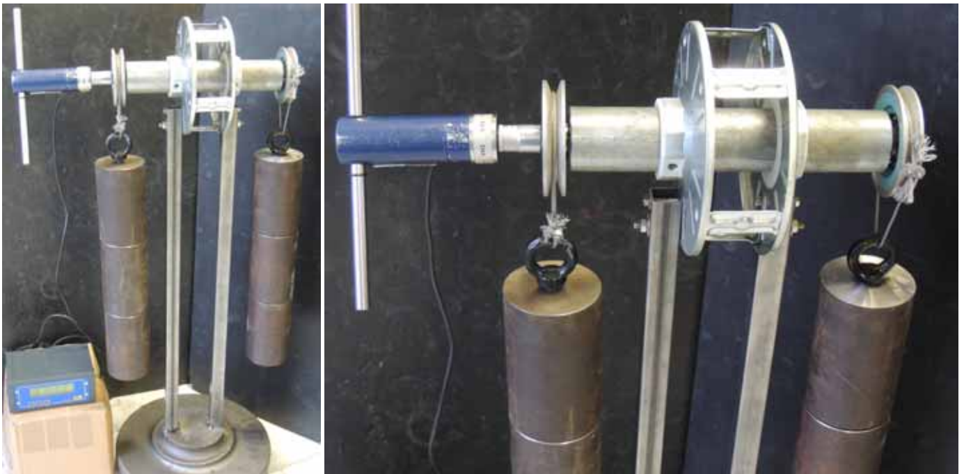
Photo N°2 – Testing apparatus
